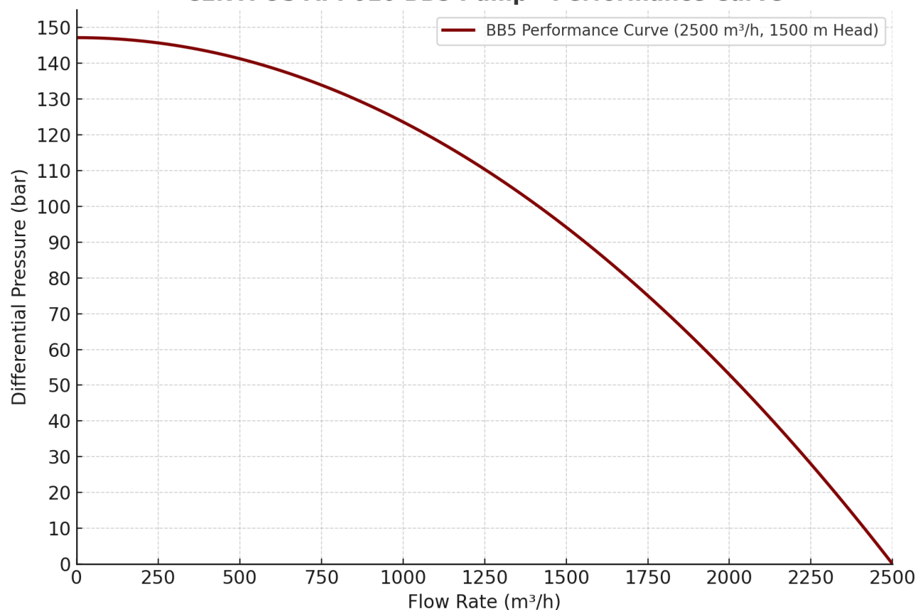
CENTFOS API 610 BB5 Pump - Performance Curve
